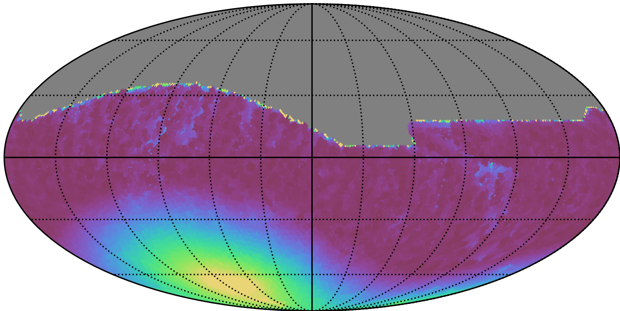
weather_cloudso16v3.4_10yrs All sky i band: Min moonDistance
