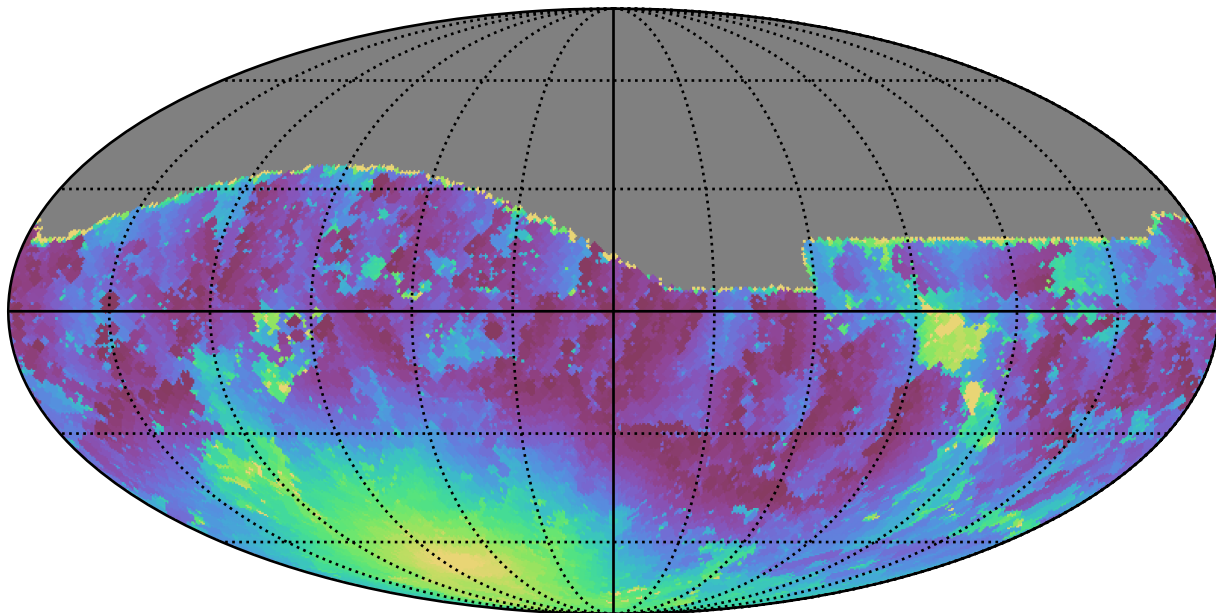
weather_cloudso16v3.4_10yrs All sky g band: Min moonDistance
