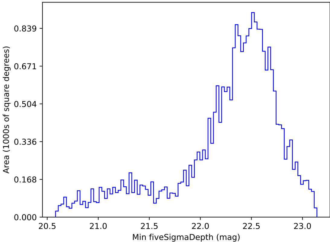
weather_cloudso16v3.4_10yrs Yr 1 z band: Min fiveSigmaDepth
