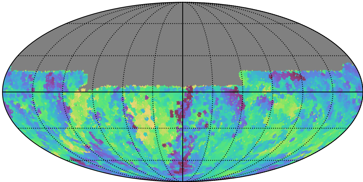
weather_cloudso16v3.4_10yrs Yr 1 y band: Min fiveSigmaDepth
