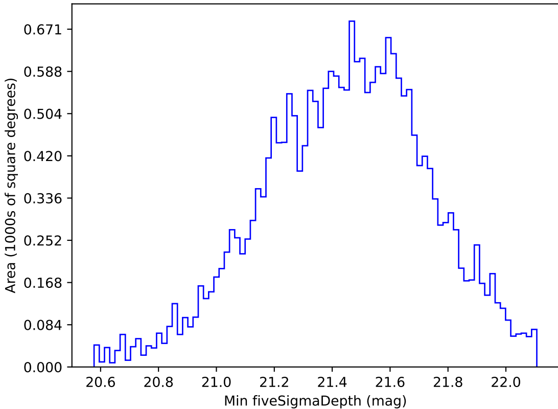
weather_cloudso16v3.4_10yrs Yr 1 y band: Min fiveSigmaDepth
