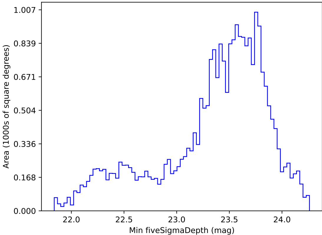
weather_cloudso16v3.4_10yrs Yr 1 r band: Min fiveSigmaDepth
