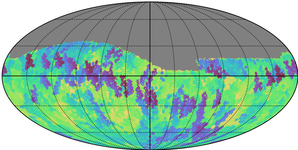
weather_cloudso16v3.4_10yrs Yr 1 i band: Min fiveSigmaDepth
