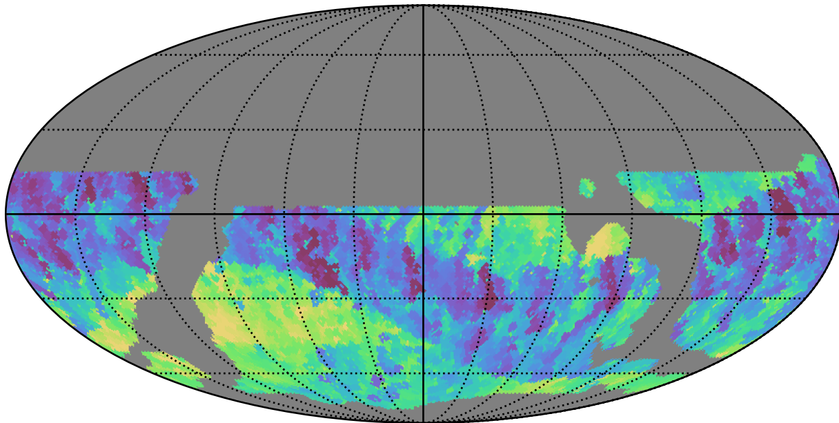
weather_cloudso16v3.4_10yrs WFD z band: Min fiveSigmaDepth
