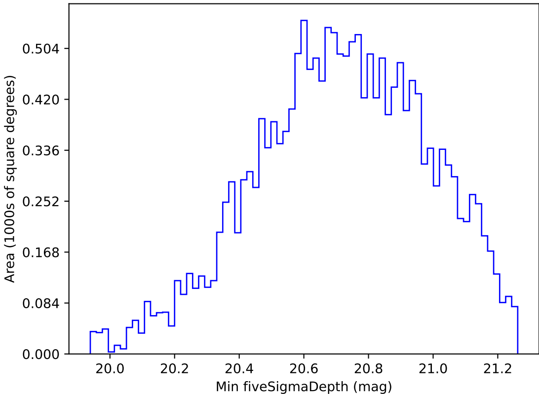
weather_cloudso16v3.4_10yrs WFD y band: Min fiveSigmaDepth
