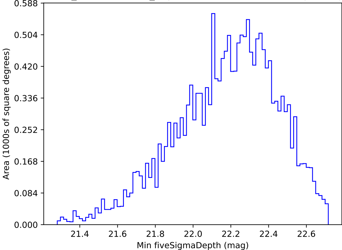
weather_cloudso16v3.4_10yrs WFD u band: Min fiveSigmaDepth
