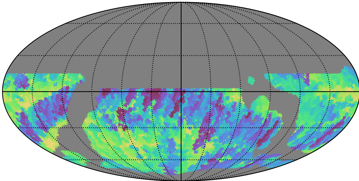
weather_cloudso16v3.4_10yrs WFD r band: Min fiveSigmaDepth
