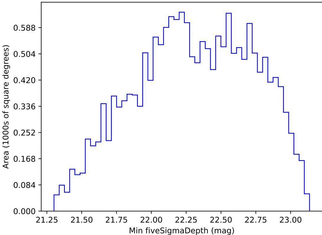
weather_cloudso16v3.4_10yrs WFD r band: Min fiveSigmaDepth
