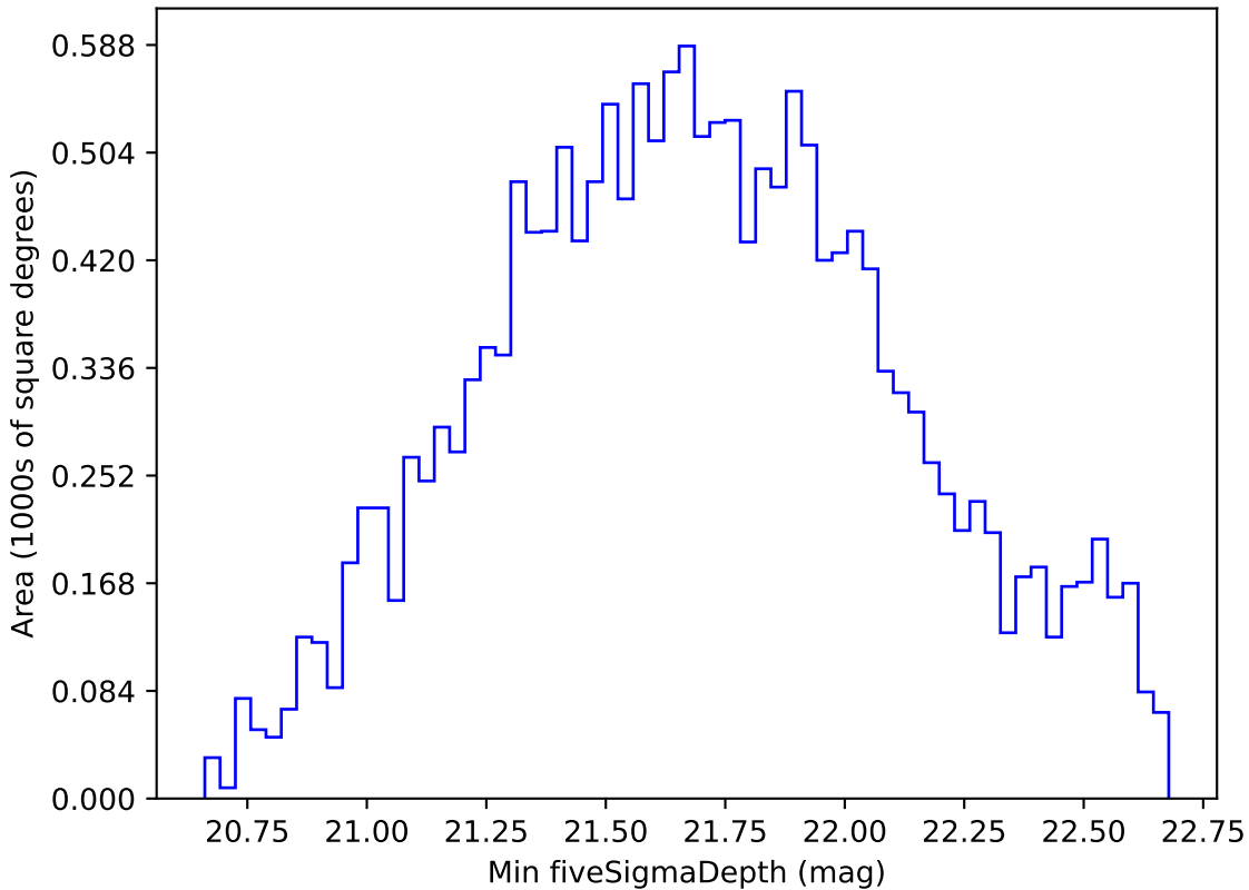
weather_cloudso16v3.4_10yrs WFD i band: Min fiveSigmaDepth
