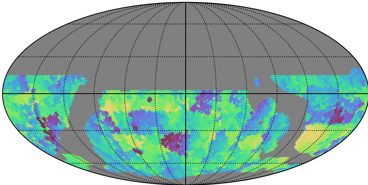
weather_cloudso16v3.4_10yrs WFD g band: Min fiveSigmaDepth
