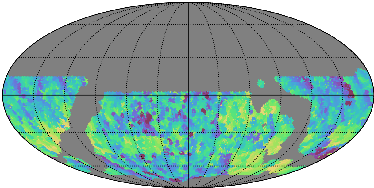
weather_cloudso16v3.4_10yrs WFD all bands: Min fiveSigmaDepth
