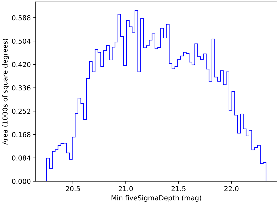
weather_cloudso16v3.4_10yrs All sky z band: Min fiveSigmaDepth
