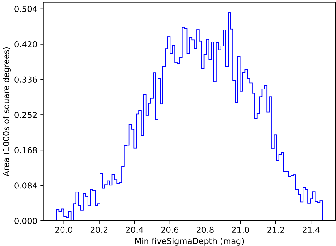
weather_cloudso16v3.4_10yrs All sky y band: Min fiveSigmaDepth
