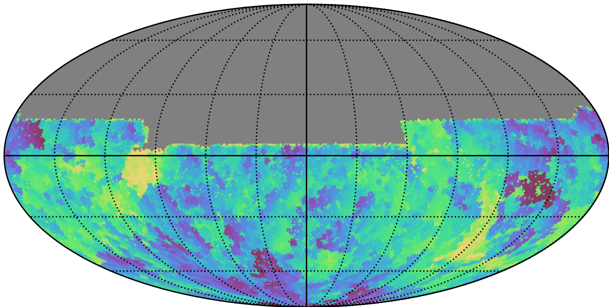
weather_cloudso16v3.4_10yrs All sky u band: Min fiveSigmaDepth
