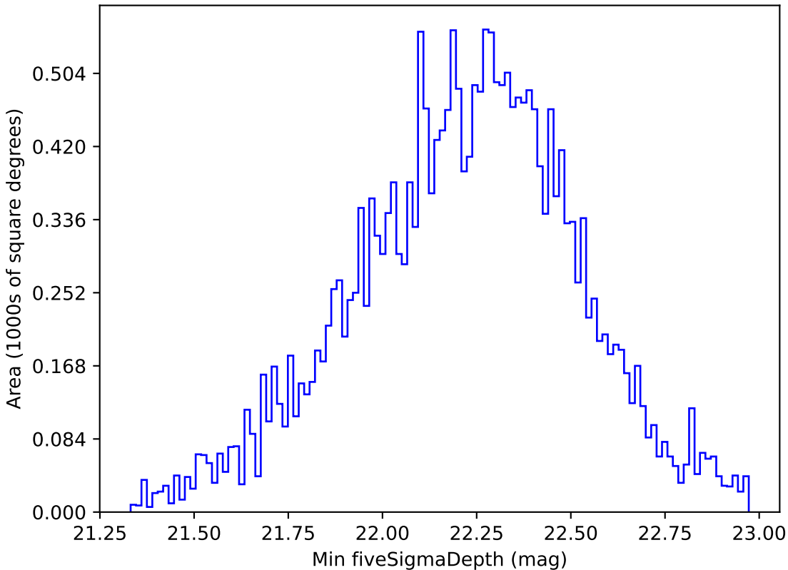
weather_cloudso16v3.4_10yrs All sky u band: Min fiveSigmaDepth
