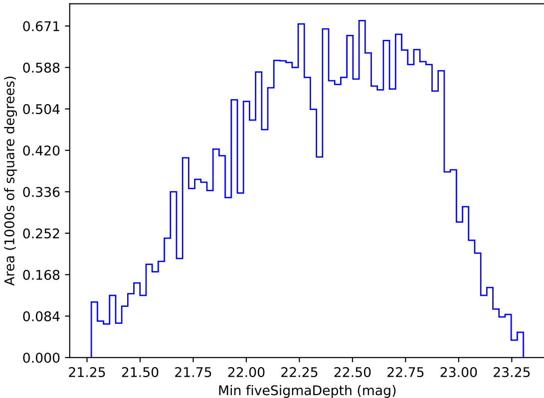
weather_cloudso16v3.4_10yrs All sky r band: Min fiveSigmaDepth
