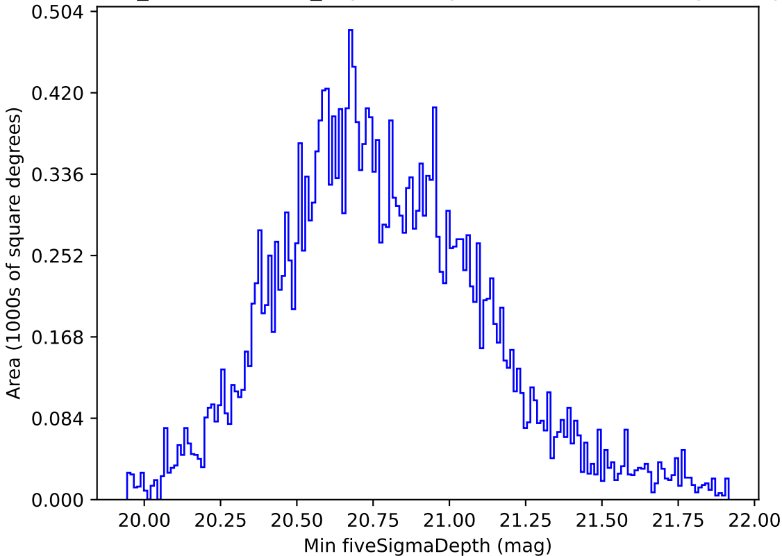
weather_cloudso16v3.4_10yrs All sky all bands: Min fiveSigmaDepth
