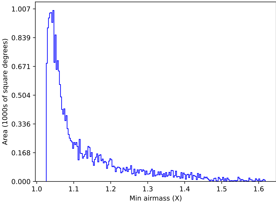
weather_cloudso16v3.4_10yrs Yr 1 y band: Min airmass
