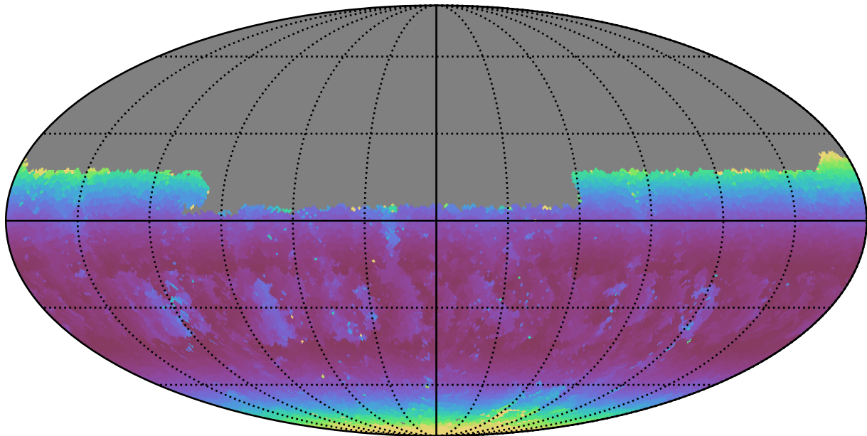
weather_cloudso16v3.4_10yrs Yr 1 u band: Min airmass
