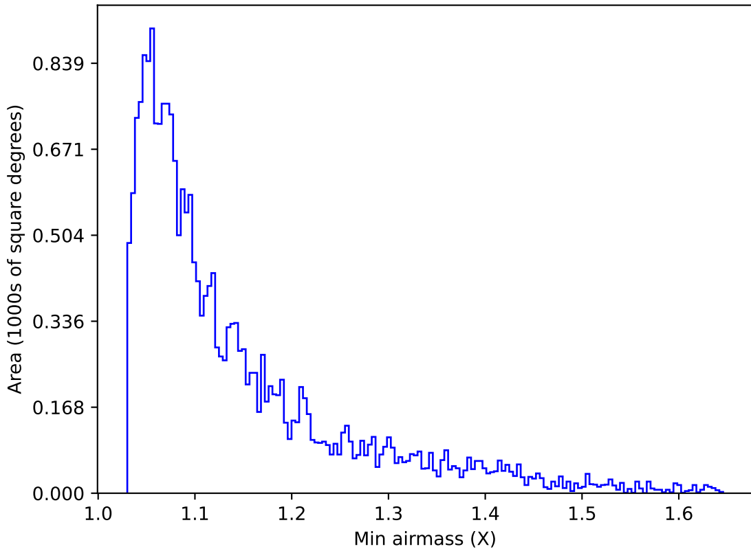
weather_cloudso16v3.4_10yrs Yr 1 u band: Min airmass
