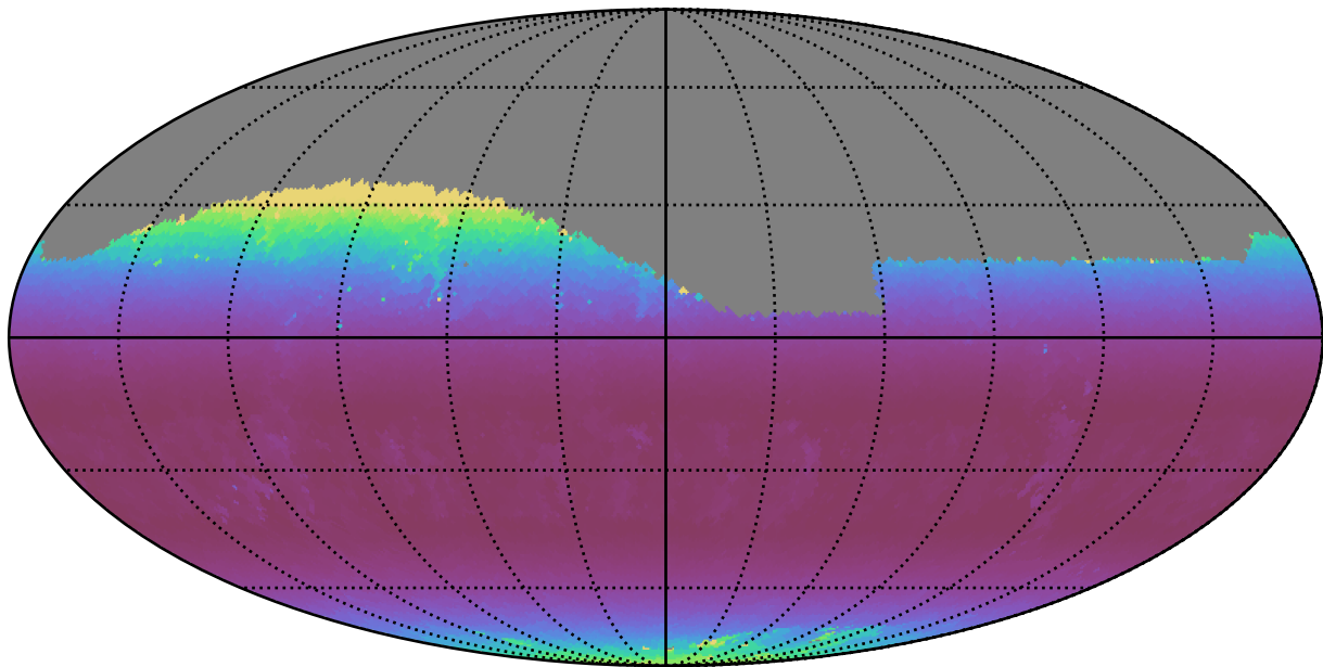
weather_cloudso16v3.4_10yrs Yr 1 r band: Min airmass
