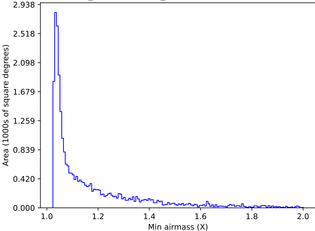
weather_cloudso16v3.4_10yrs Yr 1 i band: Min airmass
