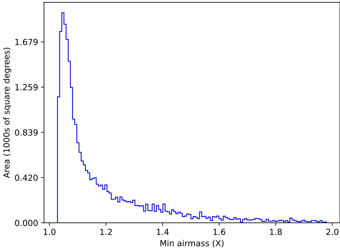
weather_cloudso16v3.4_10yrs Yr 1 g band: Min airmass
