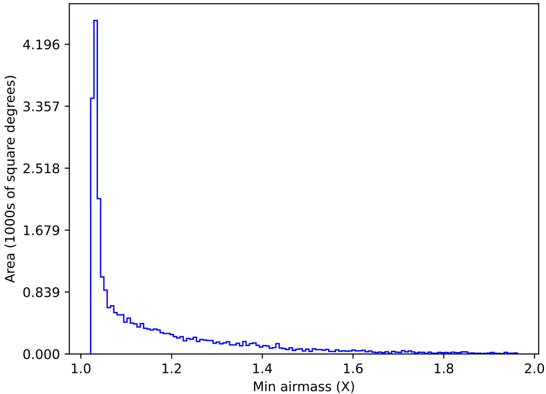
weather_cloudso16v3.4_10yrs Yr 1 all bands: Min airmass
