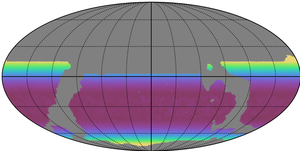
weather_cloudso16v3.4_10yrs WFD z band: Min airmass
