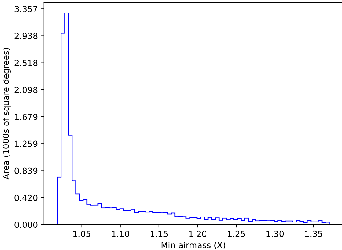
weather_cloudso16v3.4_10yrs WFD z band: Min airmass
