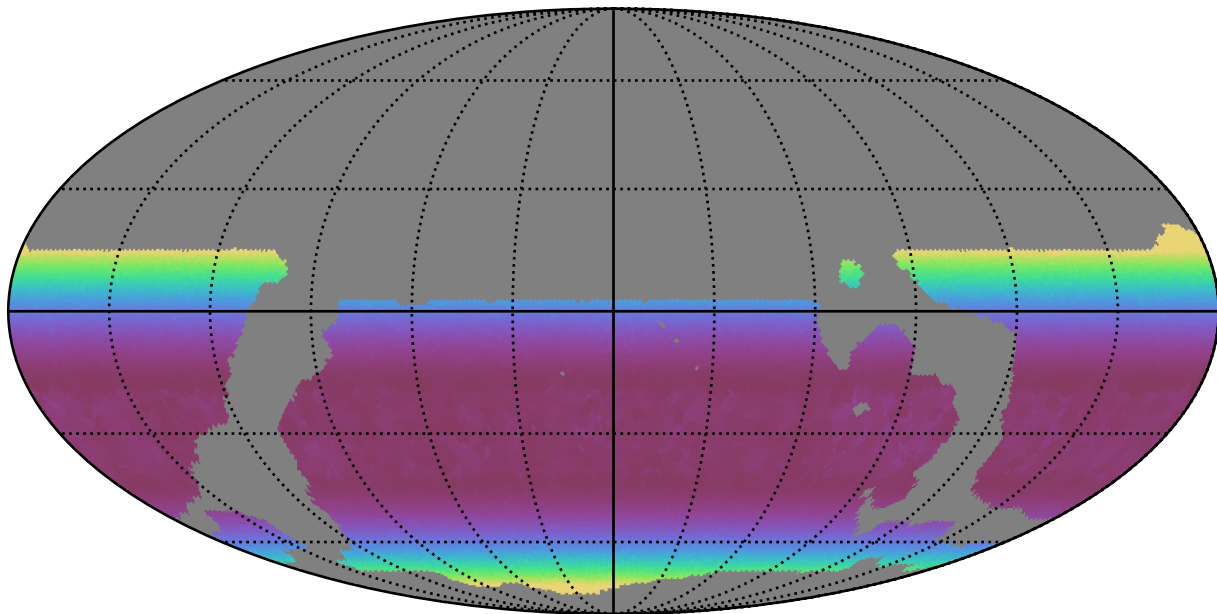
weather_cloudso16v3.4_10yrs WFD y band: Min airmass
