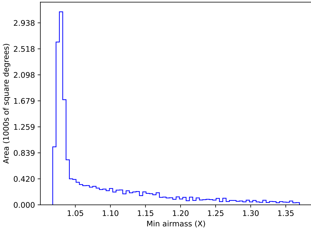
weather_cloudso16v3.4_10yrs WFD i band: Min airmass
