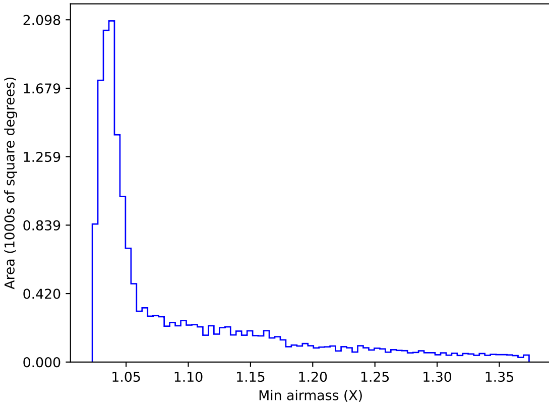
weather_cloudso16v3.4_10yrs WFD g band: Min airmass
