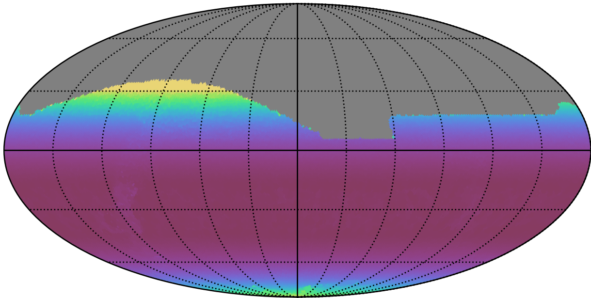
weather_cloudso16v3.4_10yrs All sky z band: Min airmass
