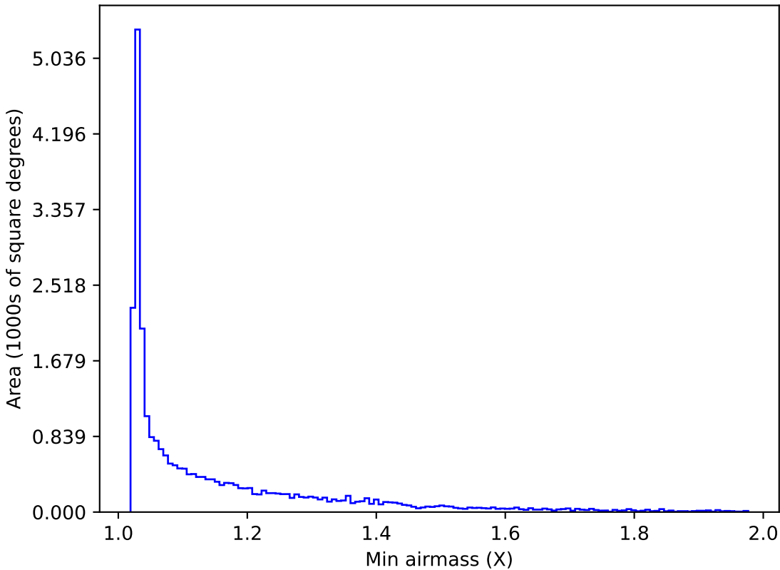
weather_cloudso16v3.4_10yrs All sky z band: Min airmass
