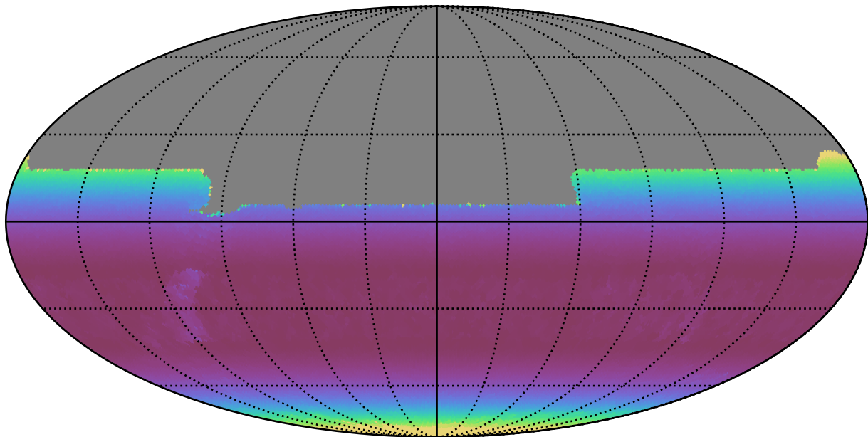
weather_cloudso16v3.4_10yrs All sky y band: Min airmass
