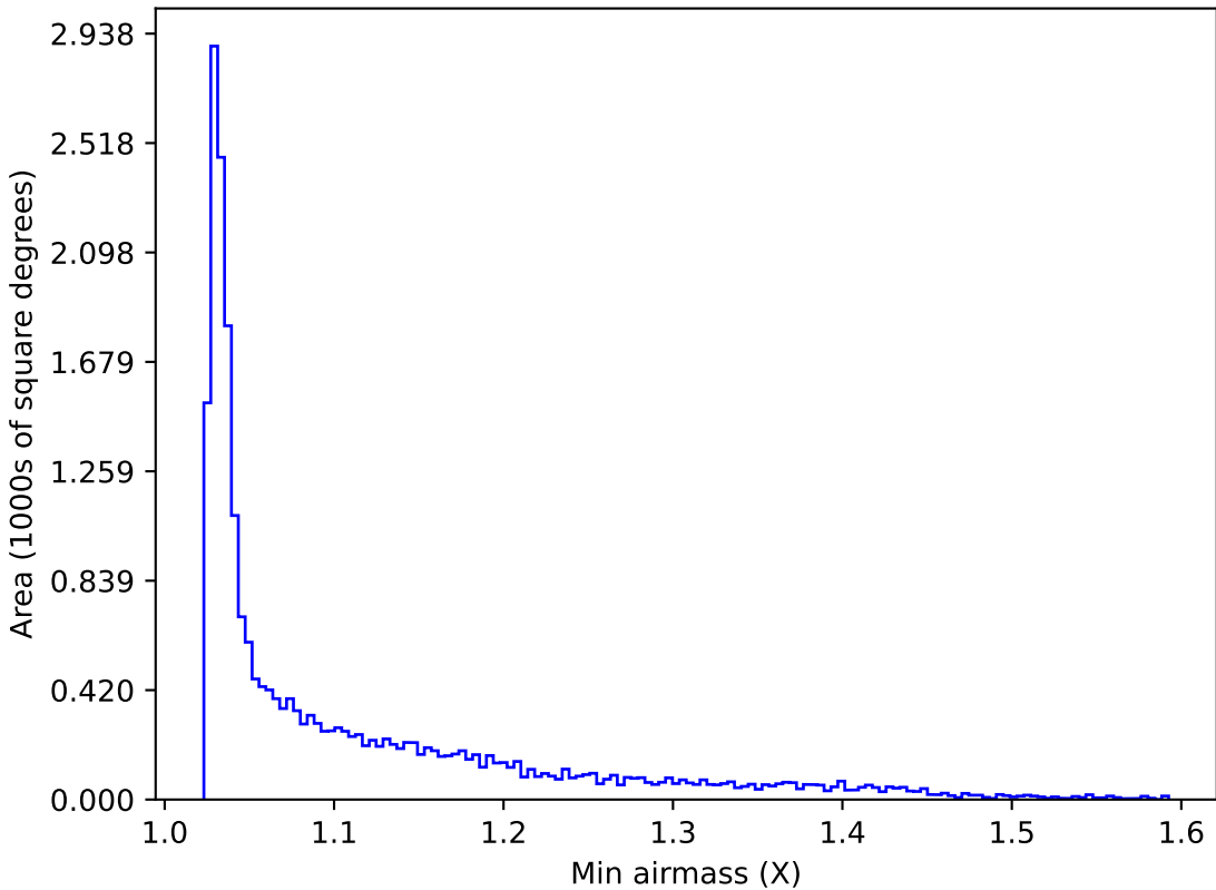
weather_cloudso16v3.4_10yrs All sky y band: Min airmass
