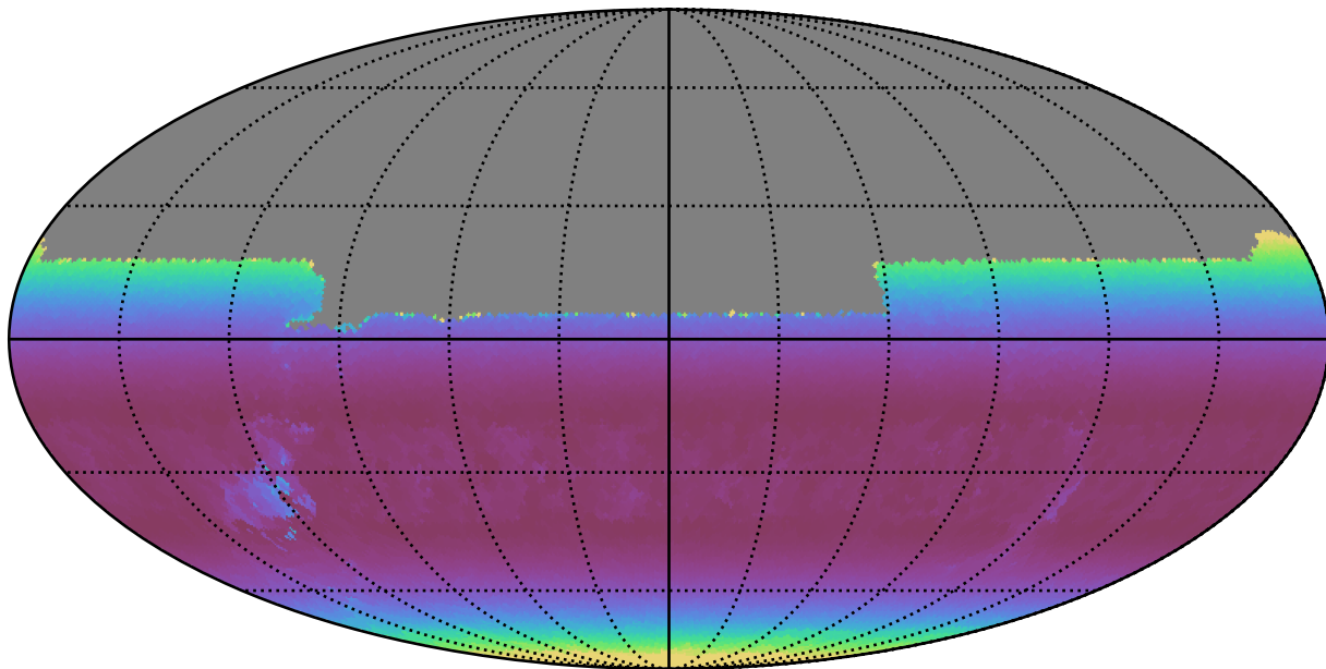
weather_cloudso16v3.4_10yrs All sky u band: Min airmass
