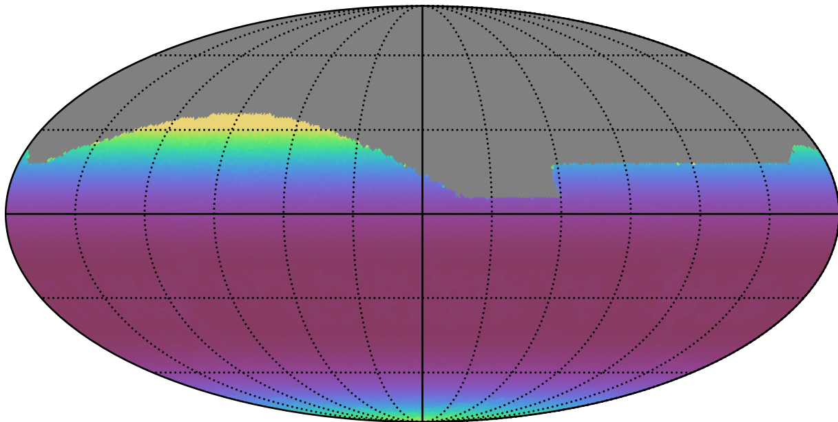
weather_cloudso16v3.4_10yrs All sky r band: Min airmass
