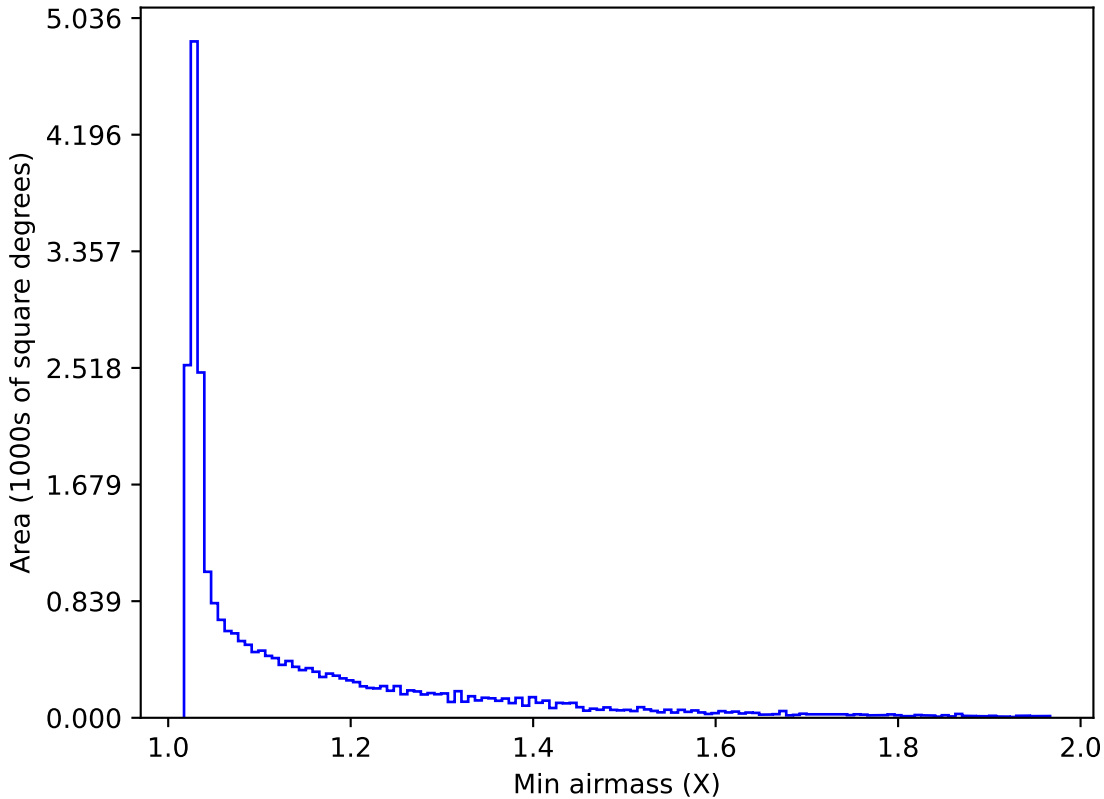
weather_cloudso16v3.4_10yrs All sky r band: Min airmass
