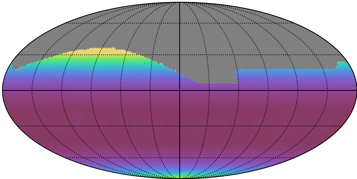
weather_cloudso16v3.4_10yrs All sky i band: Min airmass
