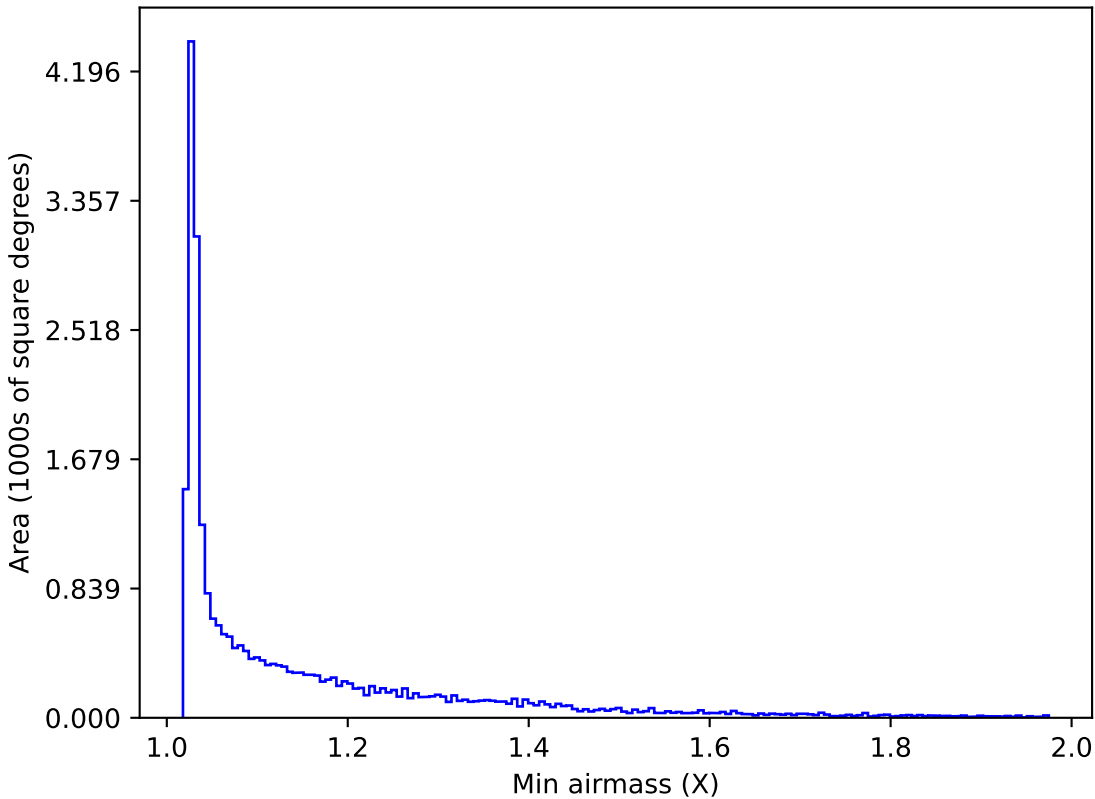
weather_cloudso16v3.4_10yrs All sky i band: Min airmass
