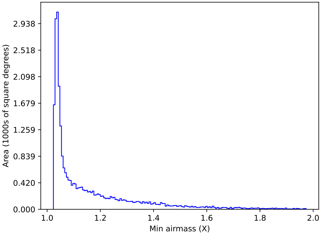
weather_cloudso16v3.4_10yrs All sky g band: Min airmass
