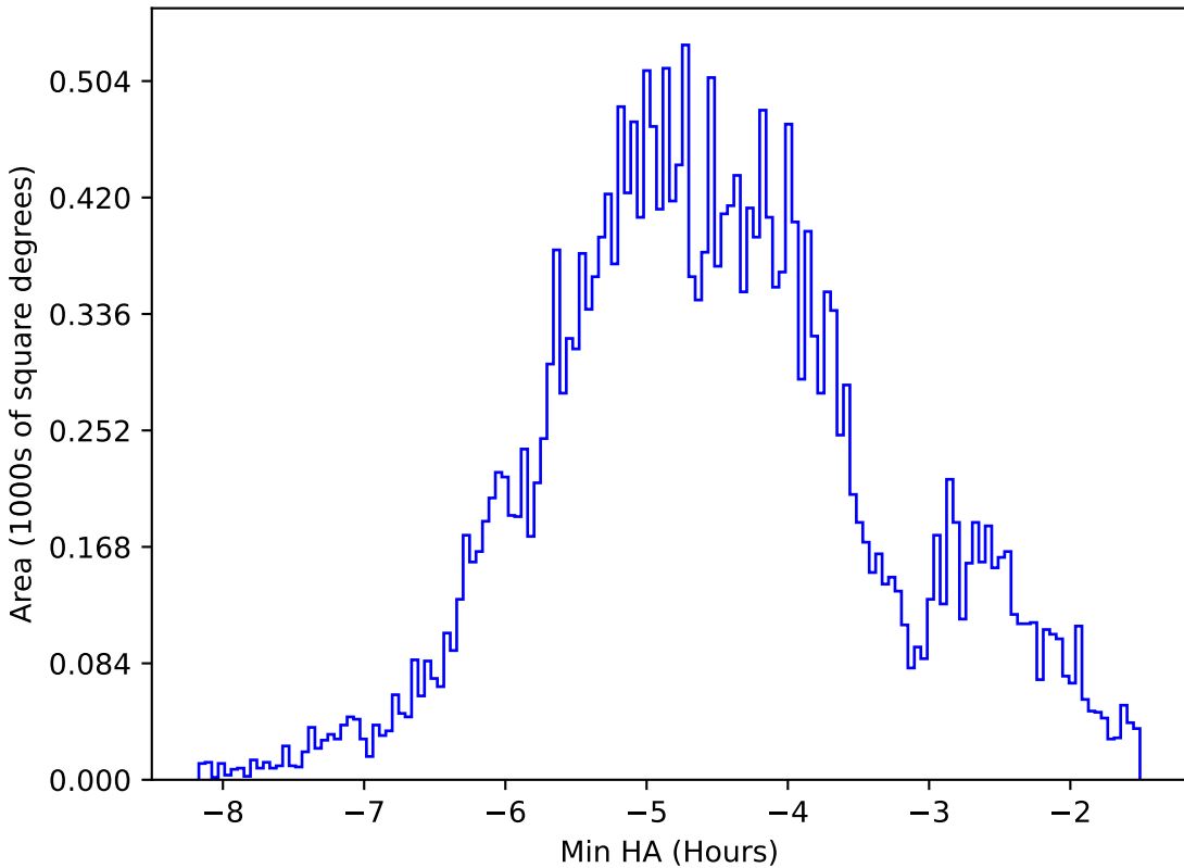
weather_cloudso16v3.4_10yrs All sky all bands: Min HA
