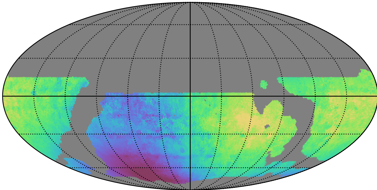
weather_cloudso16v3.4_10yrs WFD z band: Median solarElong
