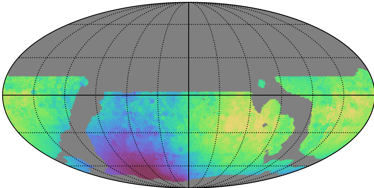
weather_cloudso16v3.4_10yrs WFD y band: Median solarElong
