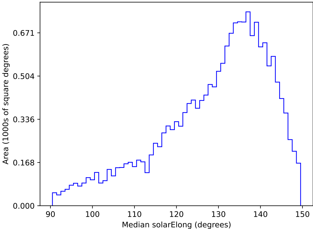
weather_cloudso16v3.4_10yrs WFD y band: Median solarElong
