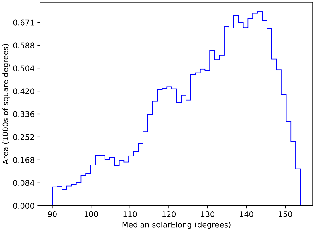
weather_cloudso16v3.4_10yrs WFD u band: Median solarElong
