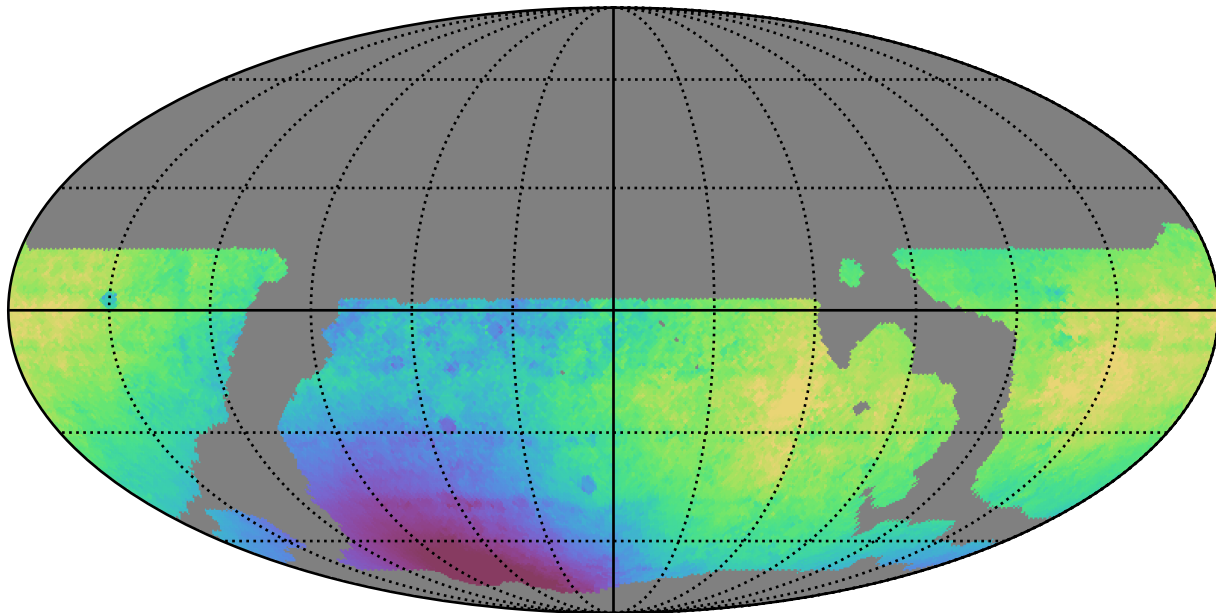
weather_cloudso16v3.4_10yrs WFD r band: Median solarElong
