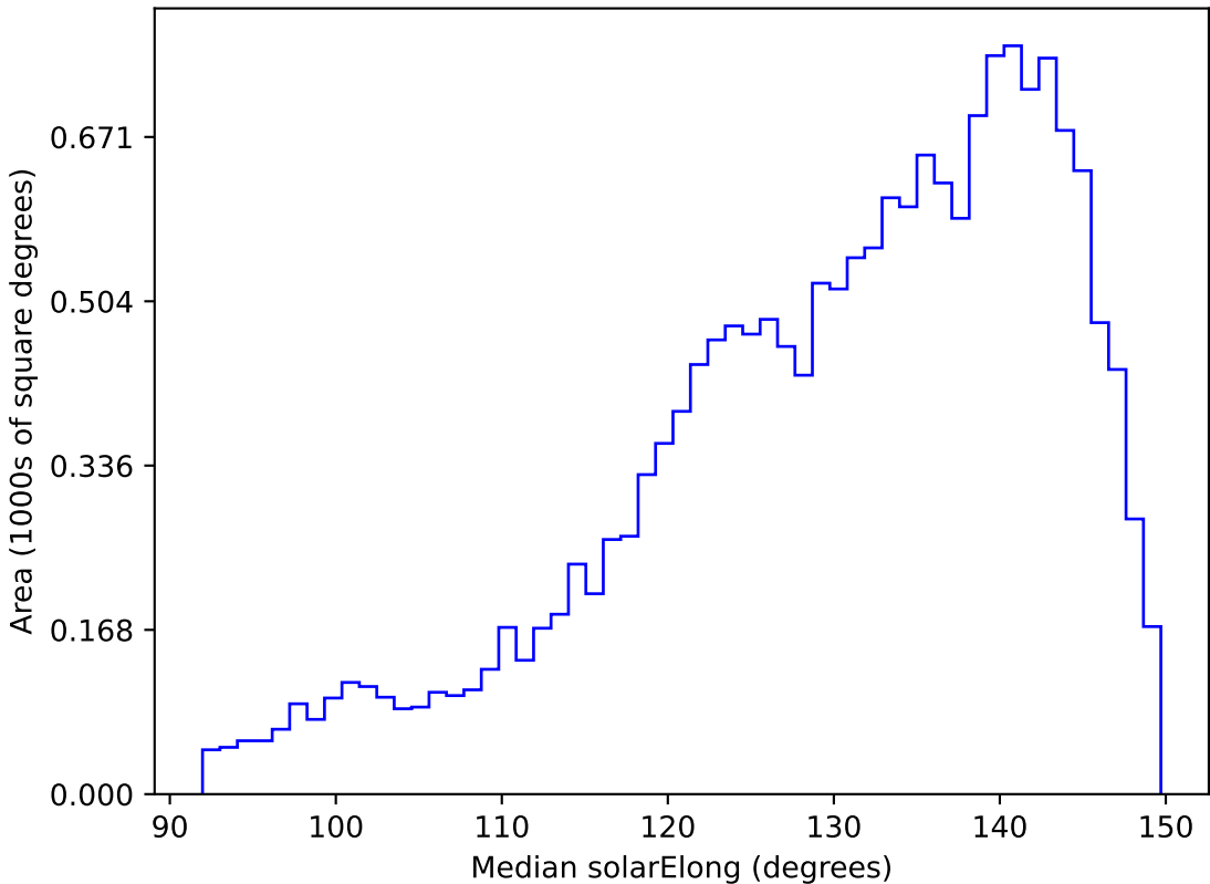
weather_cloudso16v3.4_10yrs WFD r band: Median solarElong
